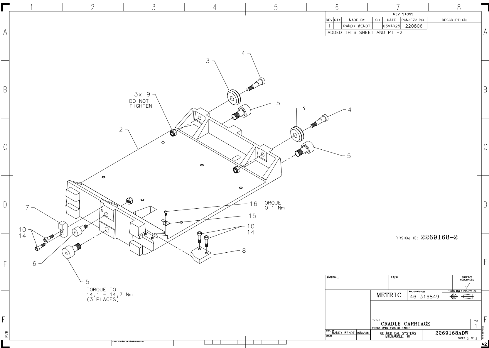
Figure 2-10 Carriage Assembly (2269168-2, sheet 2, rev1)
