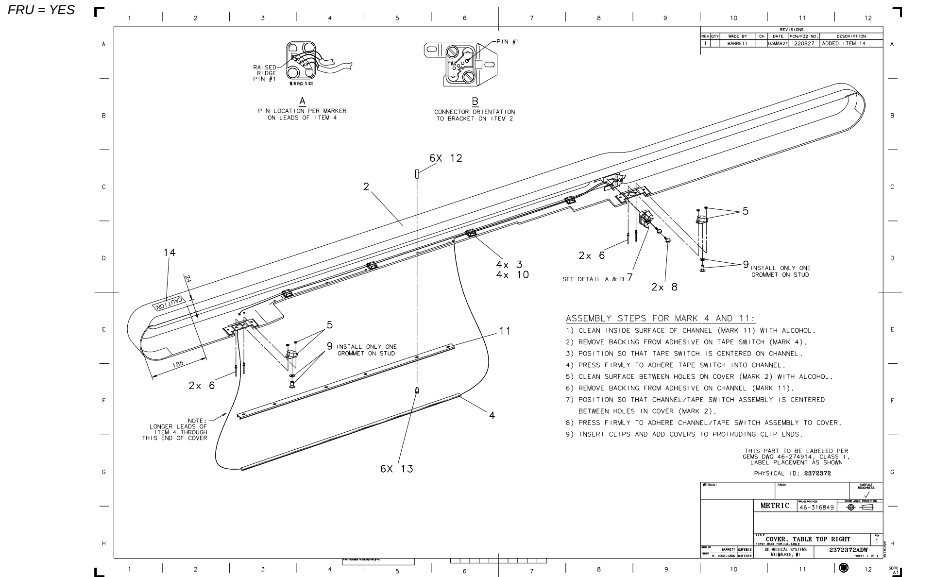
Figure 2-4 Cover Table Top - Right (2372372, sheet 1, rev 1)
