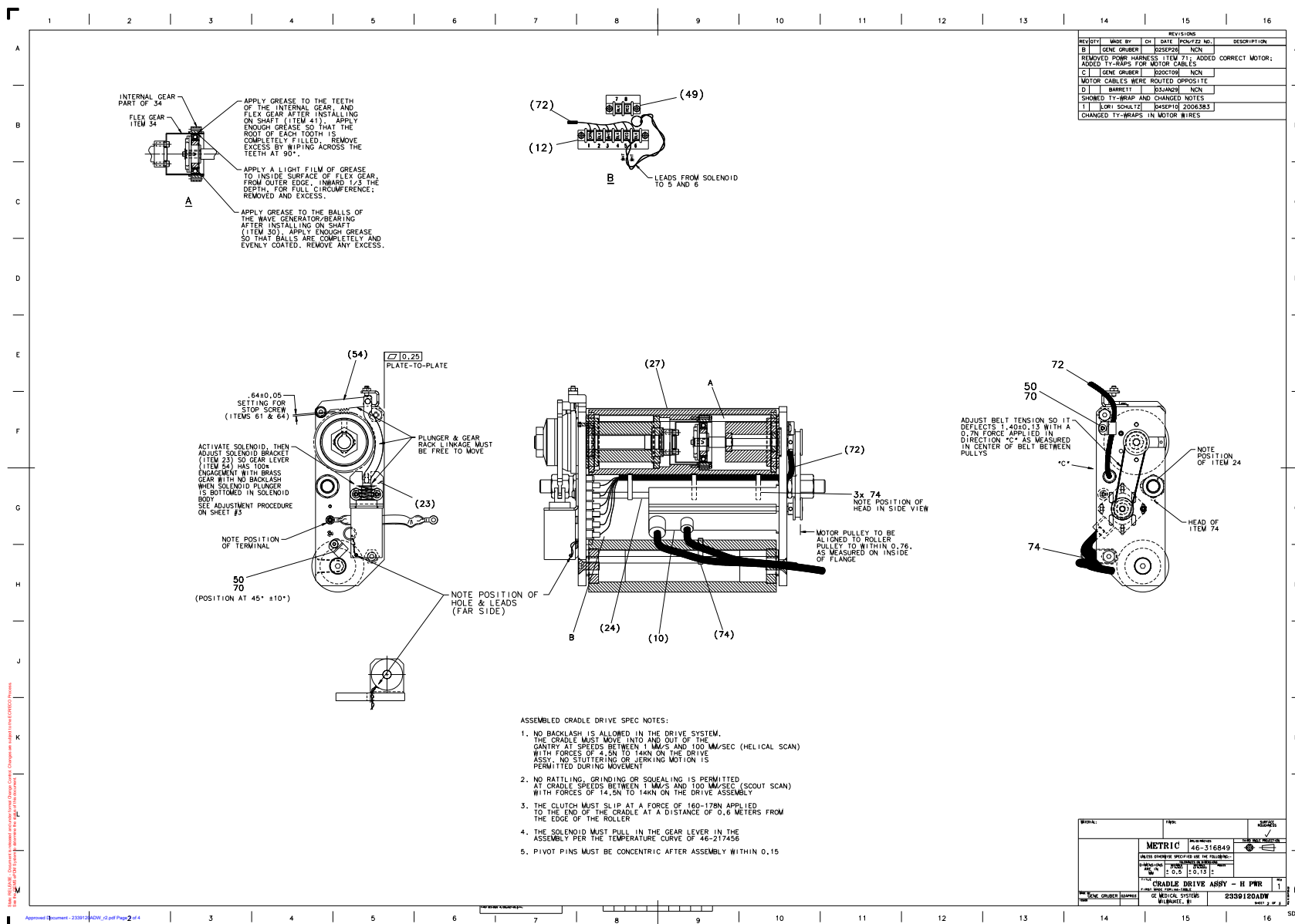
Figure 2-13 Cradle Drive Assembly (2339120, sheet 2, rev 1)
